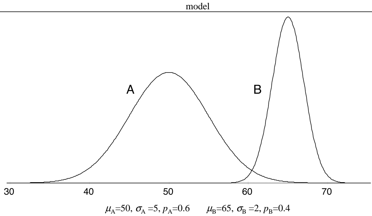
Figure 6.15 A two-class mixture model.
